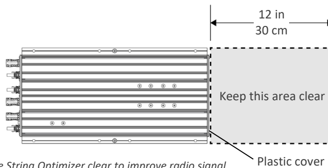
Figure 7: Keep this area of the String Optimizer clear to improve radio signal
