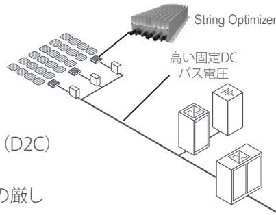
Ampt Direct-to-Converter (D2C)
