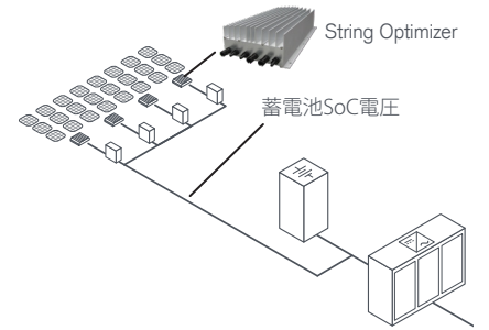
Ampt Direct-to-Battery (D2B)
