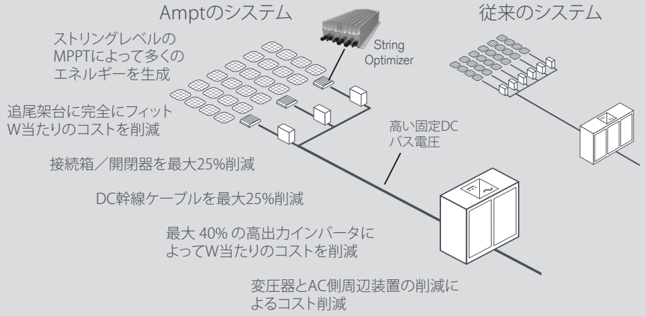
Ampt Direct-to-Converter (D2C)
